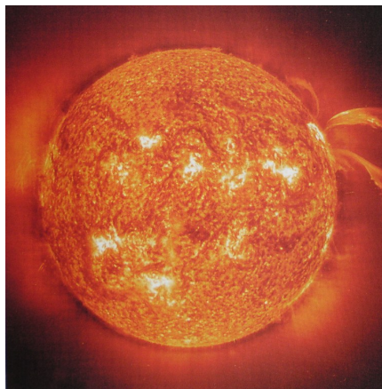
Figure 19 Sun's chromosphere shown in H alpha ( H_{\alpha} ) light (credit: universitytoday.com )
