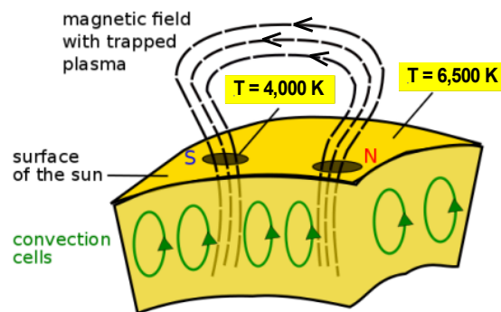
Figure 11 Formation of sunspots (credit: Sky Maps with Pierre Auger Data)
