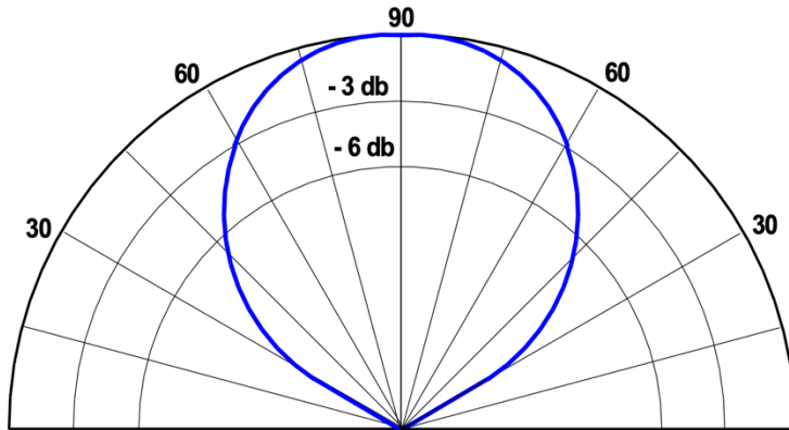
NVIS Antenna Pattern
