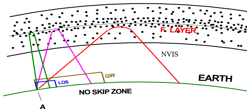
Figure 21 Local NVIS, ground wave, and line of sight propagation (source: author)
