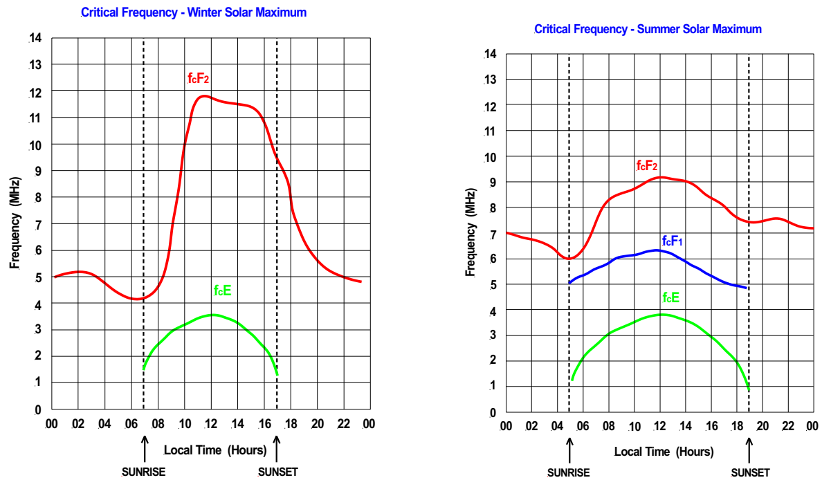
Figure 4 Critical frequency diurnal and seasonal variations (source: author)
