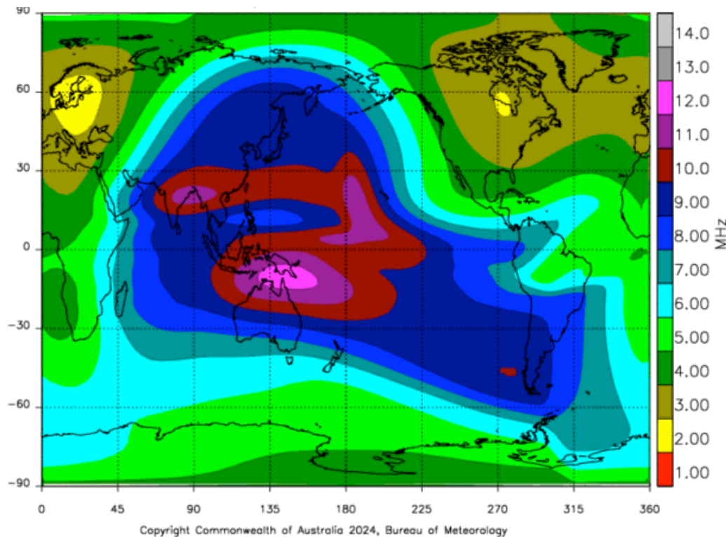
Figure 30 Critical frequency 03:00 UT January 31, 2024 (source: Australia Bureau of Meteorology)
