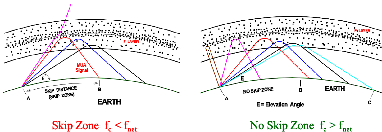
Figure 20 Local net skip distance problems (source: author)
