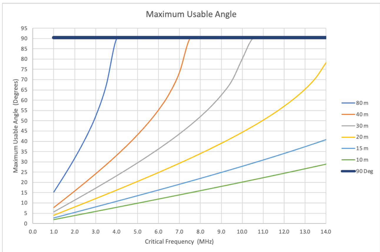
Figure 10 Maximum Usable Angle chart (source: author)
