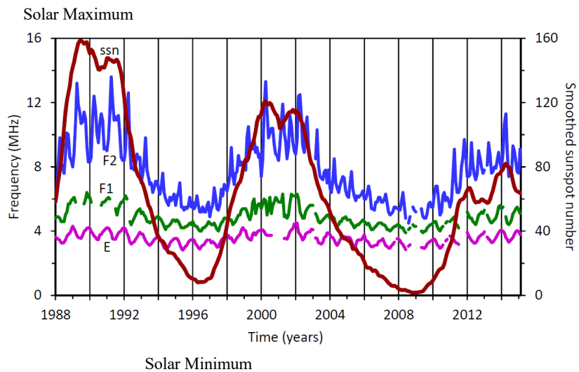
Figure 5 Critical frequency variation with the solar cycle (source: sws.bom.gov.au)
