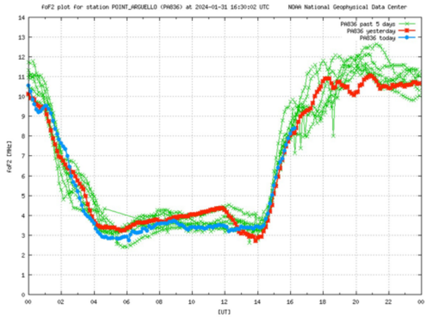
Figure 31 Point Arguello foF2 data (source: NOAA)
