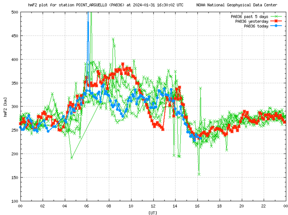
Figure 29 Ionosphere Height h_mF2 @ Point Arguello (source: NOAA)
