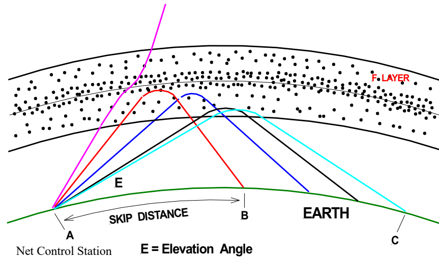
Figure 18 Regional net skip distance problem (source: author)
