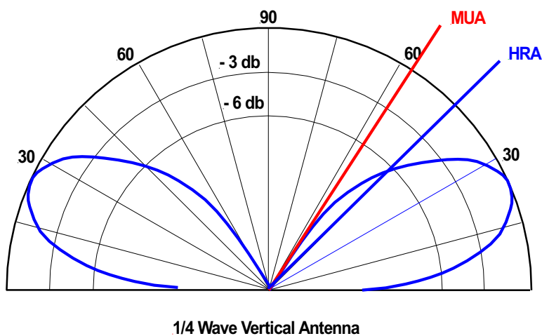
Figure 34 Vertical antenna elevation diagram (source: author)
