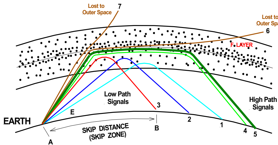
Figure 17 Hop Distance (source: author)
