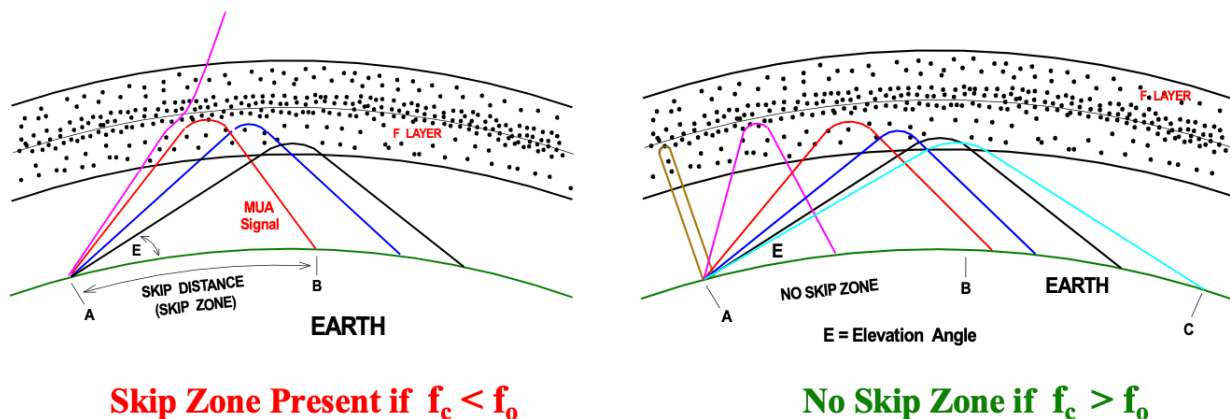
Figure 6 Skip zone presence (source: author)
