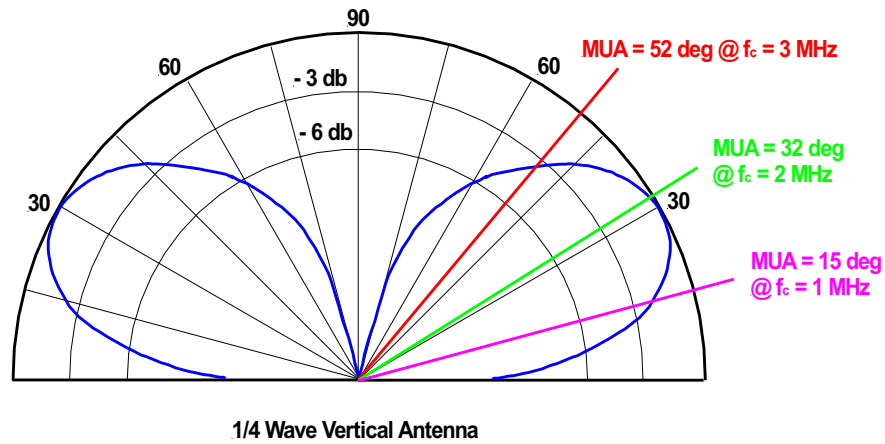
Figure 12 Radiation pattern for an 80 vertical antenna (source: author)
