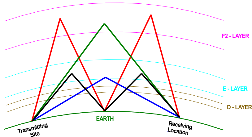
Figure 16 Signals following multiple paths to the receiving station (source: author)
