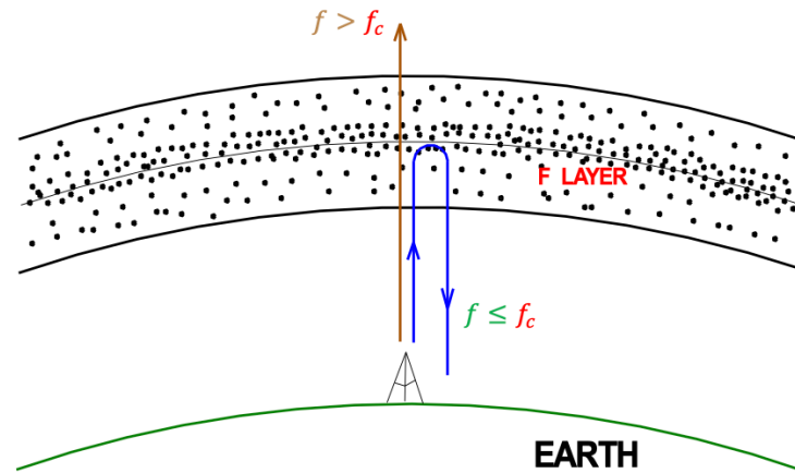
Figure 3 Critical frequency (source: author)
