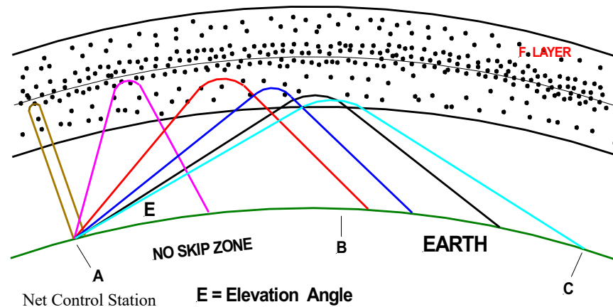
Figure 19 Regional net skip distance problem avoided (source: author)
