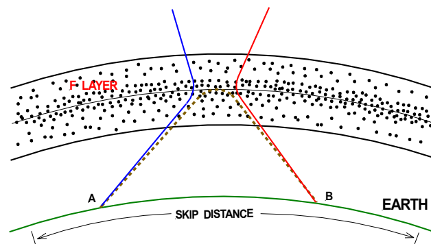
Figure 24 NVIS problems within the skip zone (source: author)
