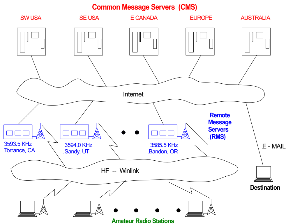
Figure 25 Winlink network (source: author)
