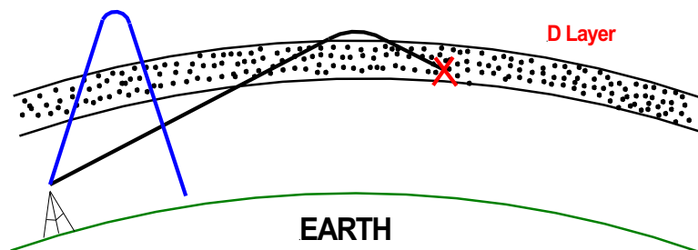
Figure 33 Long hop signal more likely to be absorbed in D layer (source: author)
