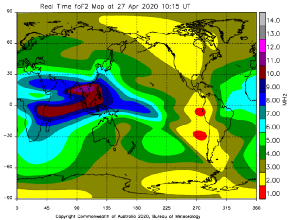
Figure 13 Typical high critical frequencies during solar minimum
