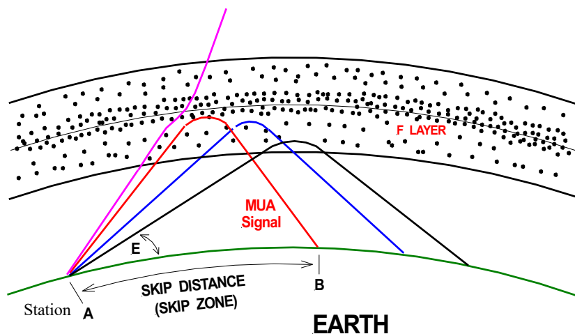
Figure 1 Skip distance and associated skip zone (source: author)
