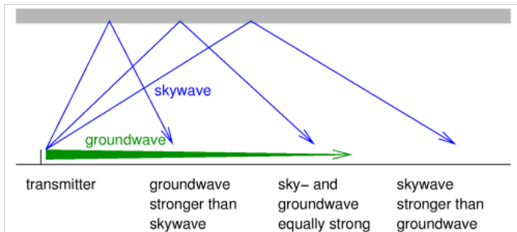
Figure 22 Skywave & ground wave multipath interference (source: PA3FWM pa3fwm@amsat.org )
