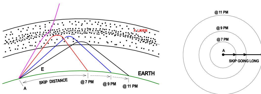
Figure 7 Skip going long (source: author)
