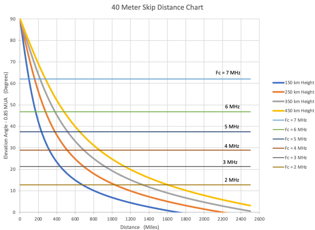
Figure 28 Skip distance chart for 40 meters (source: author)
