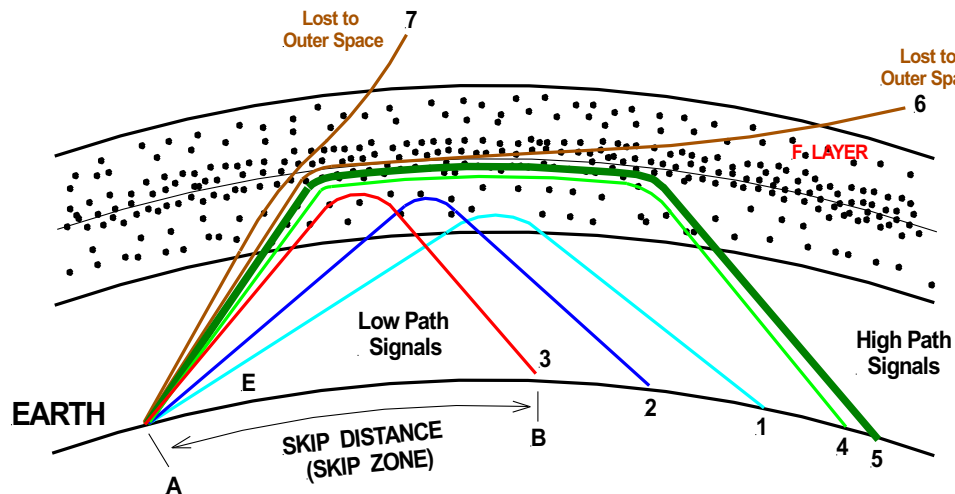
Figure 14 Hop Distance (source: author)
