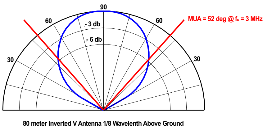
Figure 11 Radiation pattern for an 80 Inverted-V antenna (source: author)
