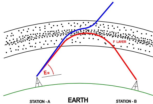
Figure 9 Maximum Usable Angle (source: author)
