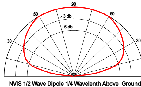
Figure 15 NVIS antenna floods most of the sky with RF energy (source: author)
