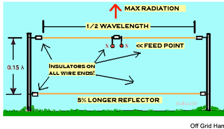
Figure 32 Two element NVIS antenna
