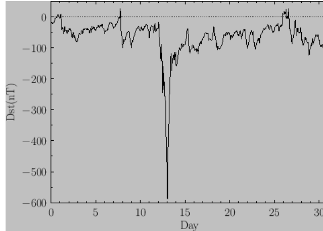
Figure 1 Dst index for the month of March 1989 (source: Farside.ph.utexas.edu)
