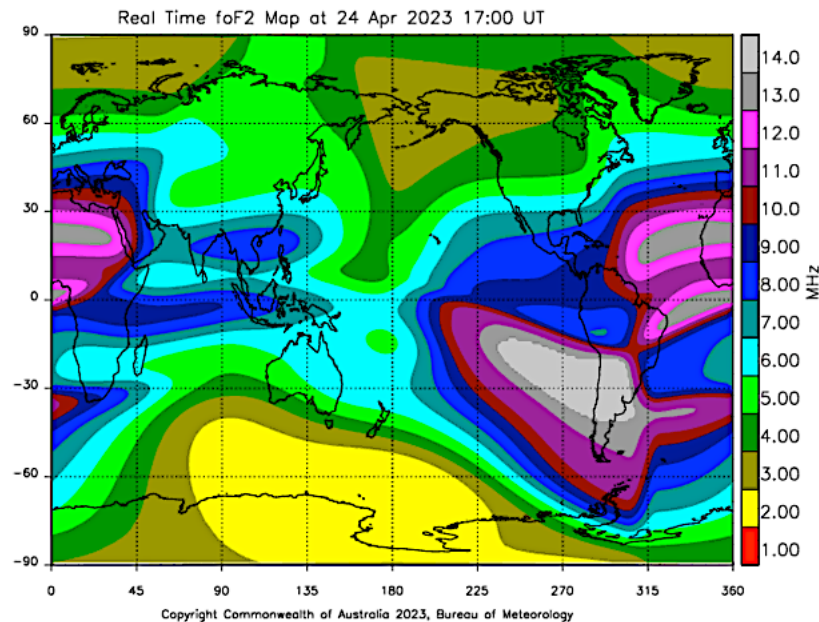
Figure 23 Critical frequency map during a solar wind storm
